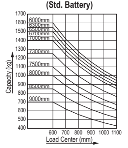
CAPACITY CHART
